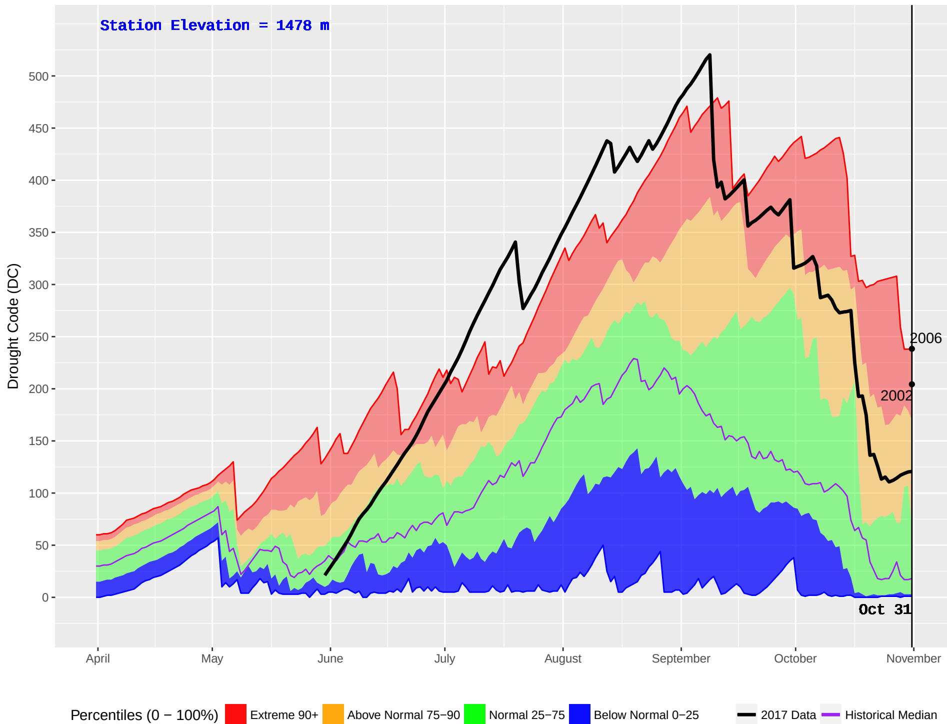
BERRY (267) : Historical (1989–2016) and Current (2017) Noon Drought Code (DC)
