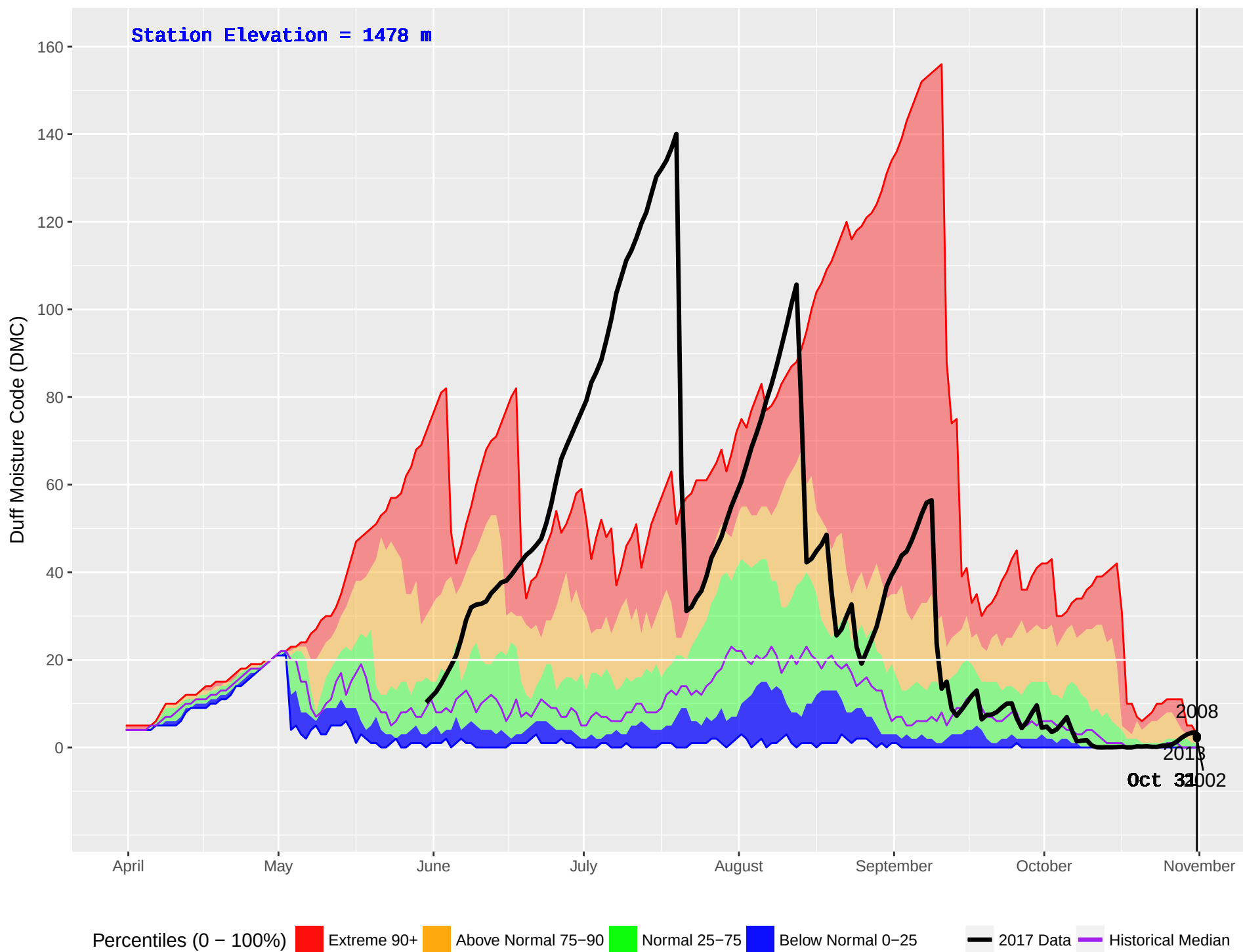
BERRY (267) : Historical (1989–2016) and Current (2017) Noon Duff Moisture Code (DMC)
